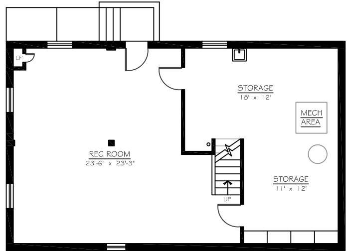
LOWER LEVEL
