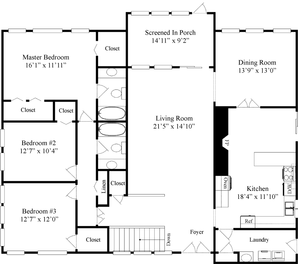
Main Level
